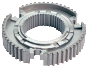
Synchroniser rings
