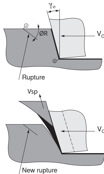
Source: chip formation according to Ackerschott, Berkold
