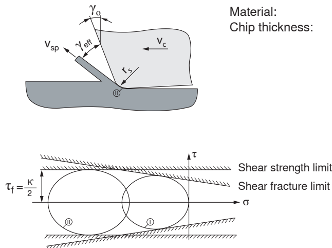
Source: chip formation for small chip thicknesses (according to Kaiser), tension/stress condition according to Siebel, Kloos, Berkold, Kaiser
