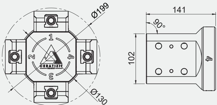
Technical Drawings
