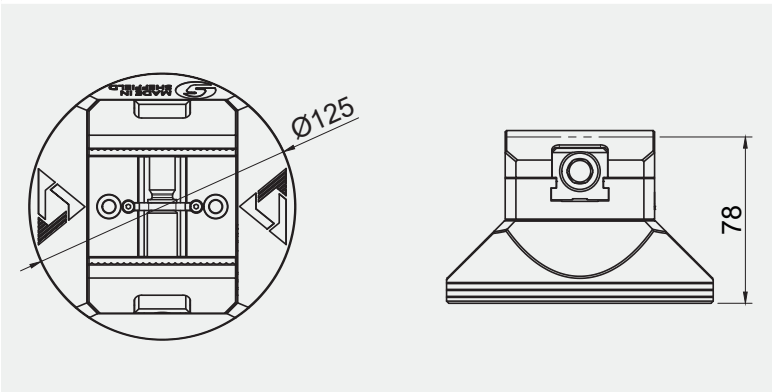
Technical Drawings
