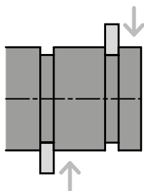
External grooving
