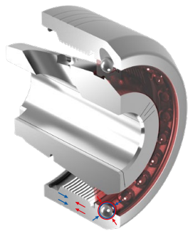
Conventional deep-groove ball bearings: positive engagement during clamping (red) or release (blue)
