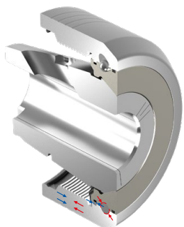
Angular ball bearings for the HDC-chuck: positive engagement during clamping (red) or release (blue)
