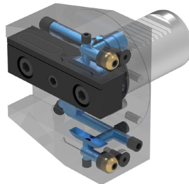
VDI square adapters – DC
