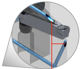
Dual cooling (rake face and flank)
