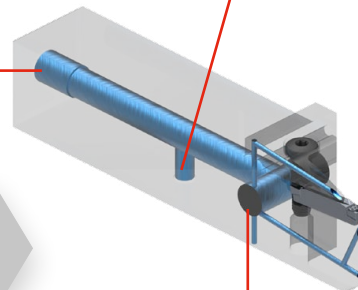
Dual cooling (rake face and flank)
