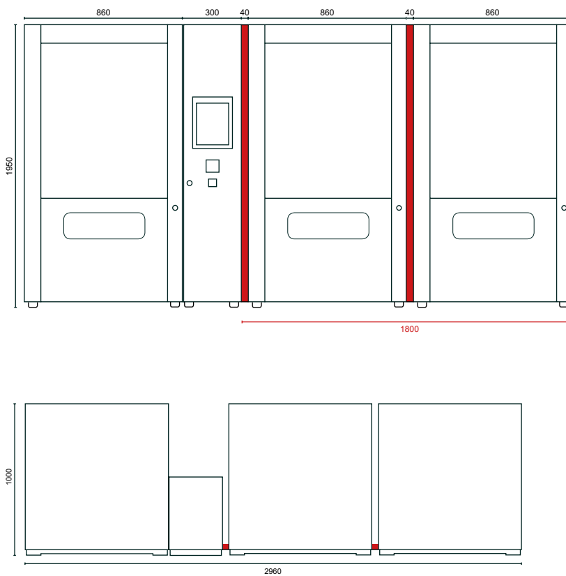
Tool-O-Mat 80 – Main Unit + Extension Unit + Extension Unit
