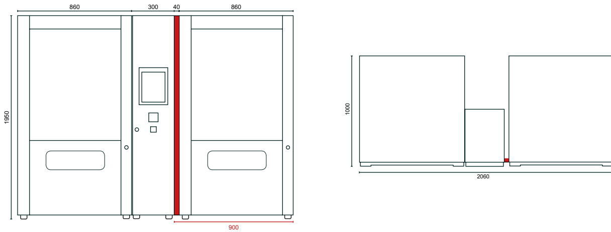
Tool-O-Mat 80 – Main Unit + Extension Unit
