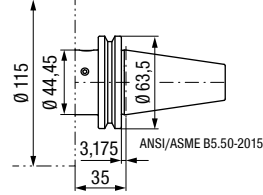
UAS-115-CAT40-...-L35 Standard
