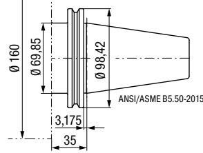
UAS-160-CAT50-...-L35 Standard
