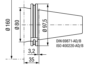
UAS-160-SK50-...-L35 Standard
