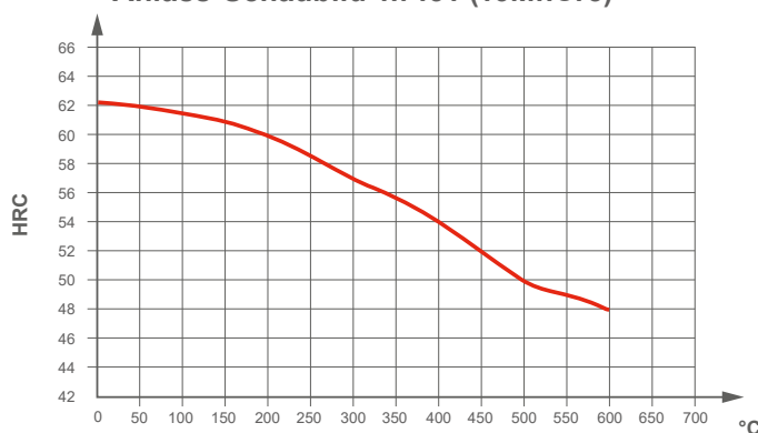
Anlass-Schaubild 1.7131 (16MnCr5)
